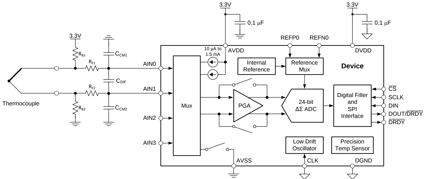
Figure 68. Thermocouple Measurement
